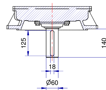
Shaft detail
